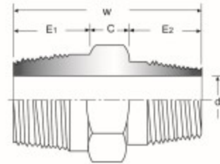
异径六角头双丝头 Reducing Hexagonal Nipple
