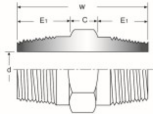
同径六角头双丝头 Straight Hexagonal Nipple
